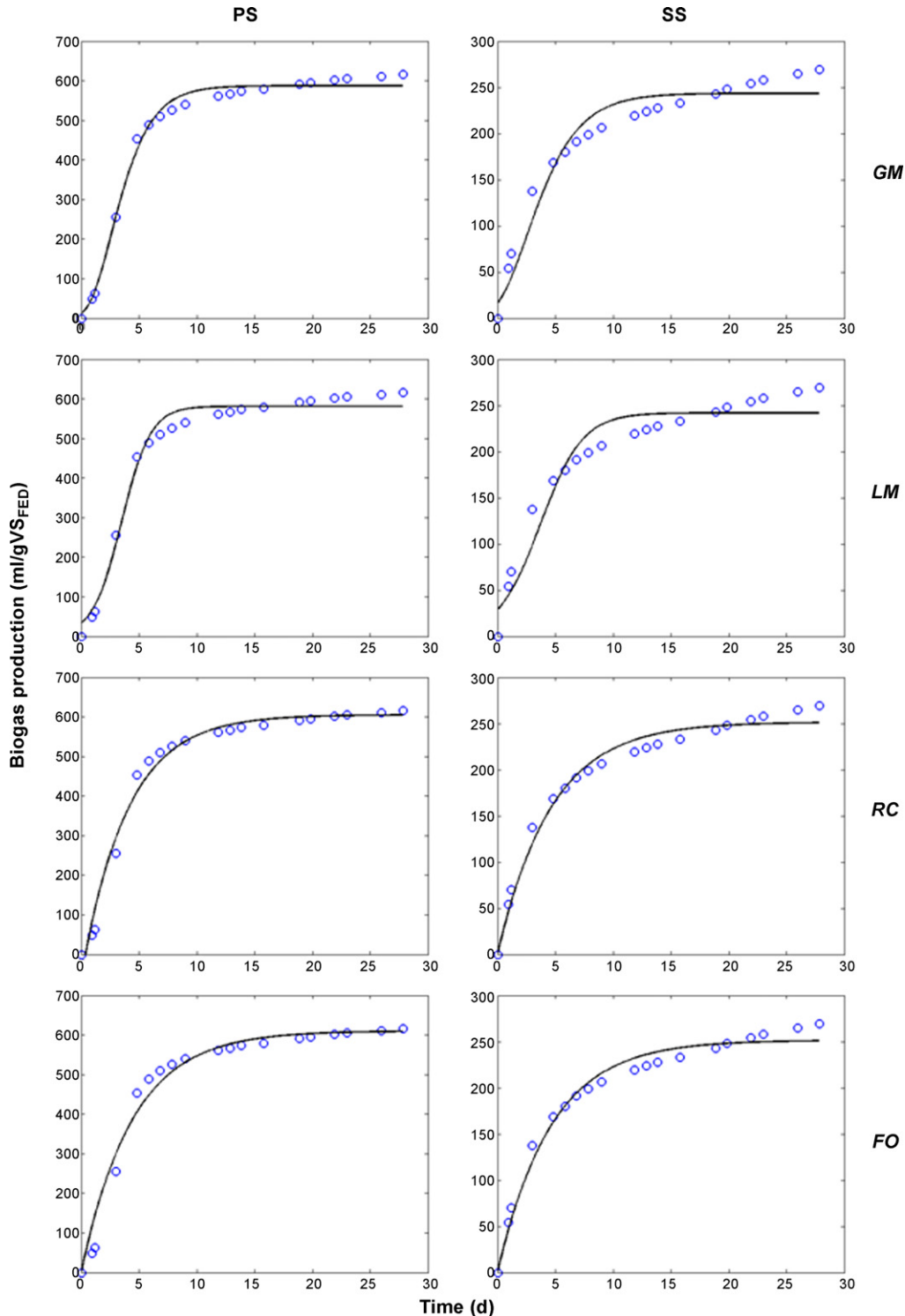
Fig. 1. Models fit with biogas production of anaerobic test using raw sludge (without pre-treatment) as substrate.
